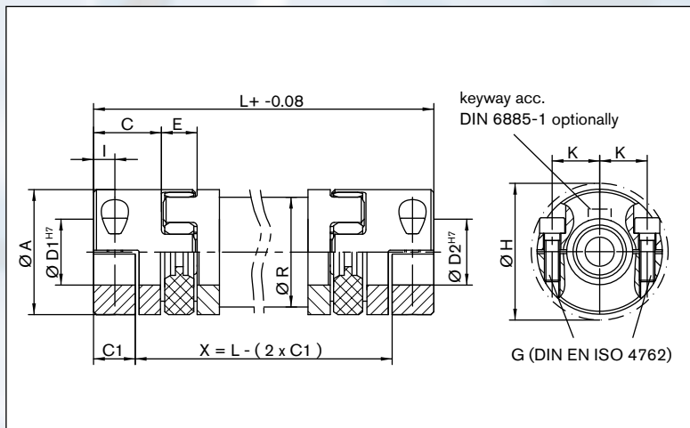
Sectional view
